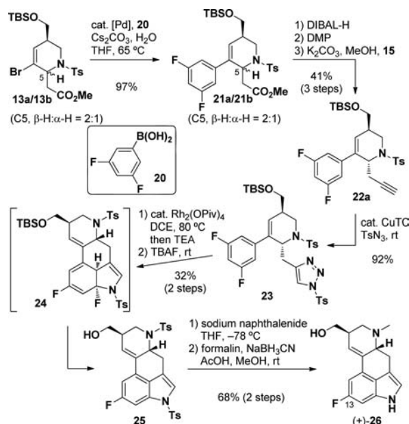
Scheme 3. Synthesis of (+)-13-Fluorolysergol ( 26 )
