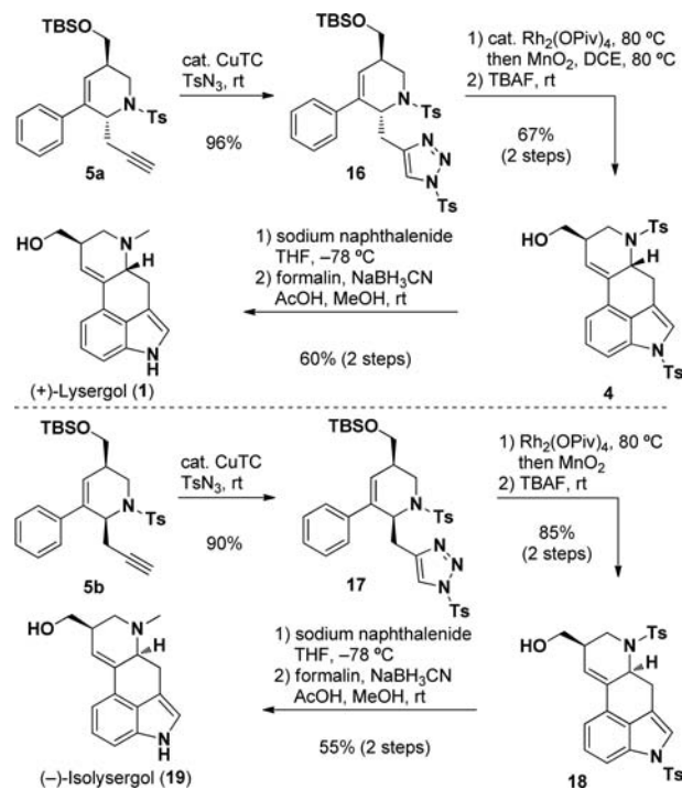
Scheme 2. Synthesis of (+)-Lysergol ( 1 ) and (–)-Isolysergol ( 19 )
