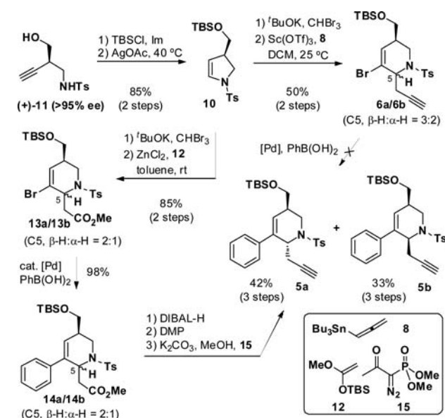
Scheme 1. Synthesis of 5a and 5b
