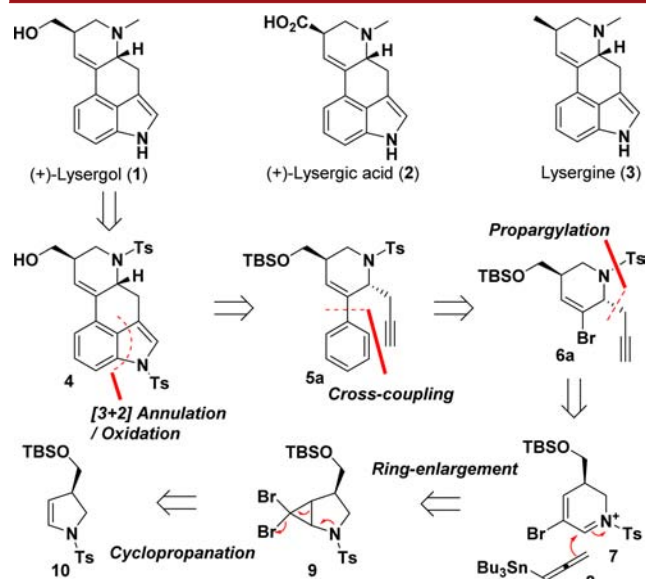
Figure 1. Retrosynthetic analysis of (+)-lysergol (1).
